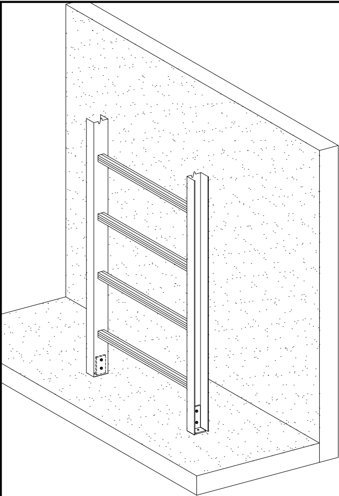
FLOOR MOUNTING BRACKET
